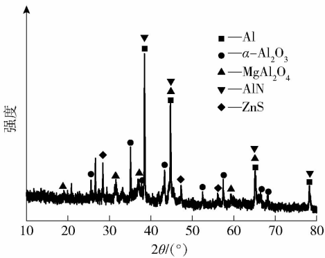
图 1 二次铝灰 XRD 图谱 Fig.1 XRD pattern of the secondary aluminum dross
