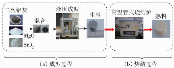
图 2 材料制备和烧结流程示意 Fig.2 Schematics of the raw materials prepared from the secondary aluminium dross
