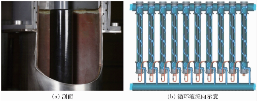
图 1 旋流电积设备示意 Fig.1 Schematic diagram of cyclone electrowinning equipment
