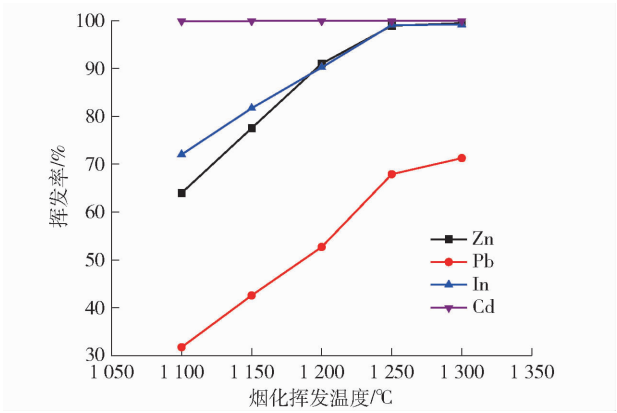
图 5 烟化挥发温度对锌、铅、铟、镉挥发率的影响 Fig. 5 Effect of fuming volatilization temperature on volatilization rate of Zn, Pb, In and Cd
