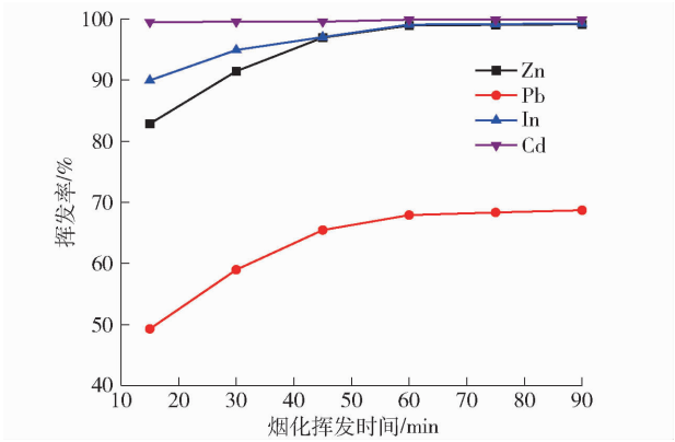
图 6 烟化挥发时间对锌、铅、铟、镉挥发率的影响 Fig. 6 Effect of fuming volatilization time on volatilization rate of Zn, Pb, In and Cd
