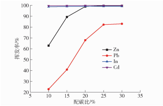
图 7 配碳比对锌、铅、铟、镉挥发率的影响 Fig. 7 Effect of carbon ratio on volatilization rate of Zn, Pb, In and Cd
