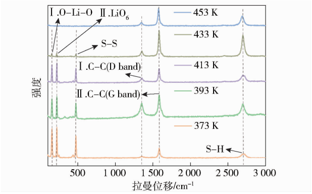
图 4 不同硫化温度下锂/石墨复合物的 Raman Fig.4 Raman spectra of lithium/graphite composites at different sulfidation temperatures
