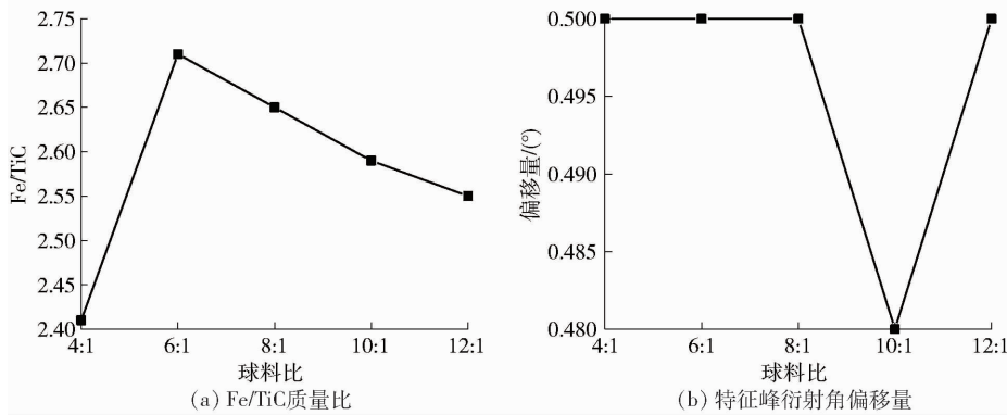
图 8 不同球料比下 Fe 与 TiC 的重量比及实际 Ti(C,N)与理论 TiC 特征峰衍射角偏移量 Fig.8 The weight ratio of Fe to TiC and the diffraction angle offset of the actual Ti(C,N) and theoretical TiC characteristic peaks under different nder different ball-to-powder ratios: (a) Fe/TiC weight ratio (b) Diffraction angle shift of characteristic peaks
