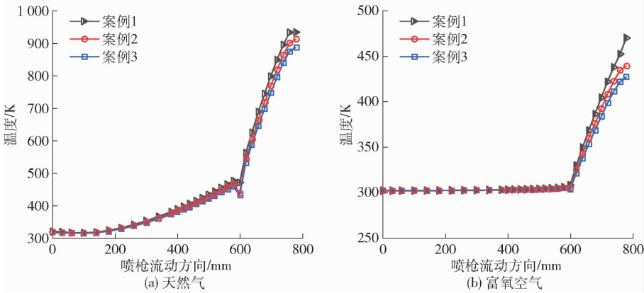
图 12 不同流量下气体温度随流动方向的变化趋势 Fig. 12 The variation of gas temperature along the flow direction at different flow rates
