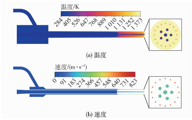
图 6 喷枪中心截面不同物理量分布云图 Fig. 6 Distribution of different physical quantities on the central cross-section of the lance
