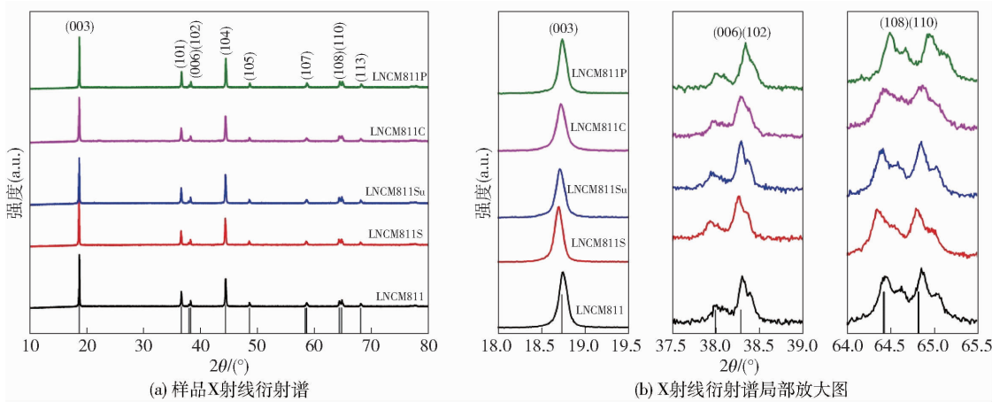
图1 样品X射线衍射谱 Fig.1 X-ray diffraction spectrums of the samples
