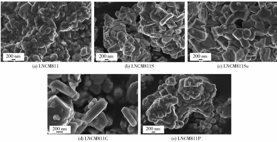
图2 样品的扫描电子显微图像 Fig.2 Scanning electron micrographs of the samples
