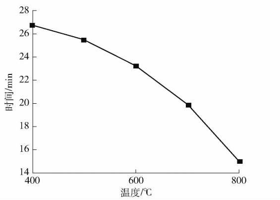
图 7 不同温度下废线路板热解耗时 Fig. 7 Pyrolysis time of waste circuit board at different temperatures
