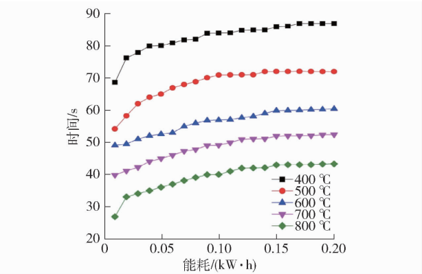
图 4 加热空坩埚时散热损失变化规律 Fig. 4 Variation law of heat loss when heating an empty crucible
