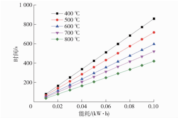
图 2 不同温度下热解炉能耗所用时间 Fig. 2 Time consumption of pyrolysis furnace at different temperatures
