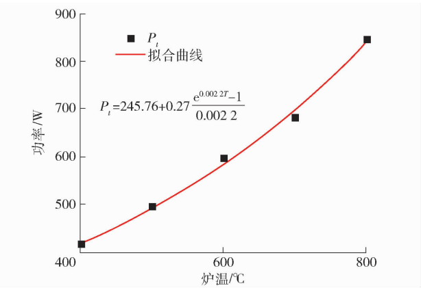
图 3 所耗功率 P_t 随炉温 T 变化 Fig. 3 Variation of consumed power P_t with furnace temperature T
