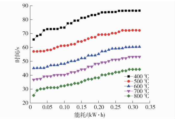
图 5 热解废线路板时散热损失变化规律 Fig. 5 Variation Law of heat loss during pyrolysis of waste circuit board
