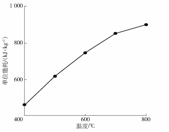
图 6 不同温度下单位废线路板热解能耗 Fig. 6 Pyrolysis energy consumption of waste circuit board at different temperatures
