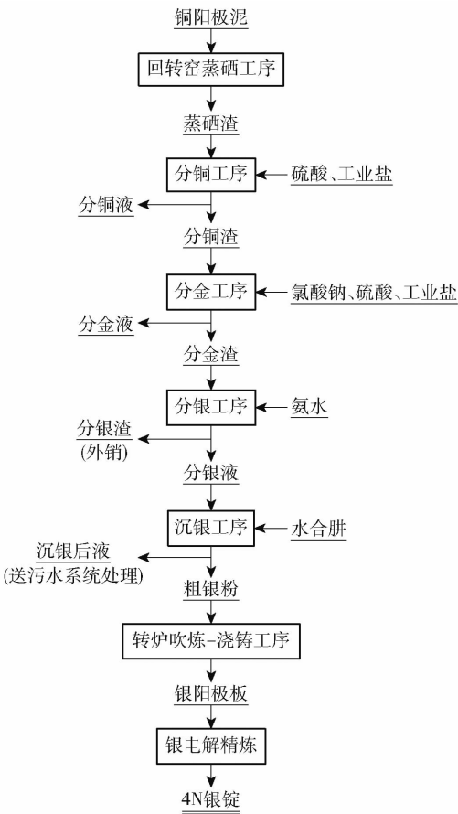
图 1 铜阳极泥提银生产工艺流程 Fig. 1 Production process flow of extracting silver from copper anode slime
