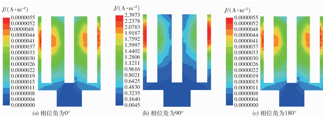
图 5 侧面上方线圈 1 Hz/1 000 AN 正弦波电流下槽内感应电流密度周期变化云图 Fig.5 Periodic variation of induced current density in the slot with 1 Hz/1000 A sinusoidal current flowing from the coil above the side
