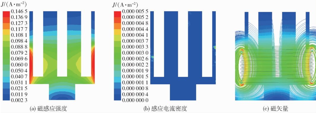
图 6 侧面下方线圈 5 000 AN 下磁感应强度、感应电流密度及磁矢量分布云图 Fig.6 Cloud map of magnetic induction intensity, induced current density and magnetic vector distribution under 5 000 AN coil at the lower side
